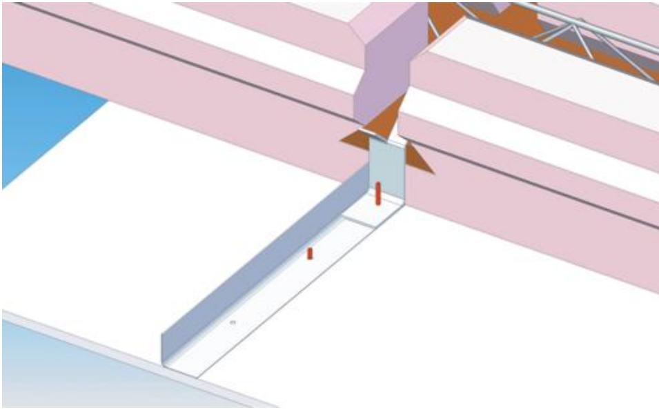
Details of construction used for mounting gypsum plates. Core plates are built in during concreting, one
